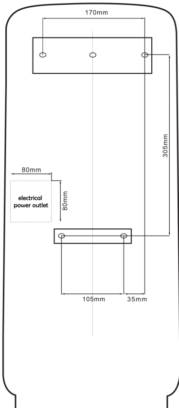
Fig. 1 drilling diagram
